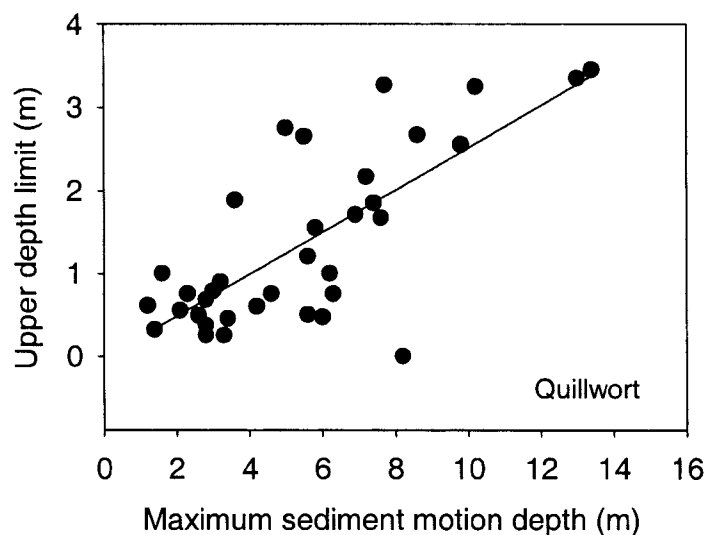
Figure 6. The relationships between (a) lower limit of LMC and (b) upper limit of quillwort vegetation and sediment motion depth.
