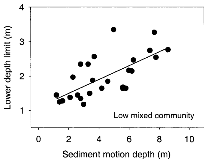
Figure 6. The relationships between (a) lower limit of LMC and (b) upper limit of quillwort vegetation and sediment motion depth.
