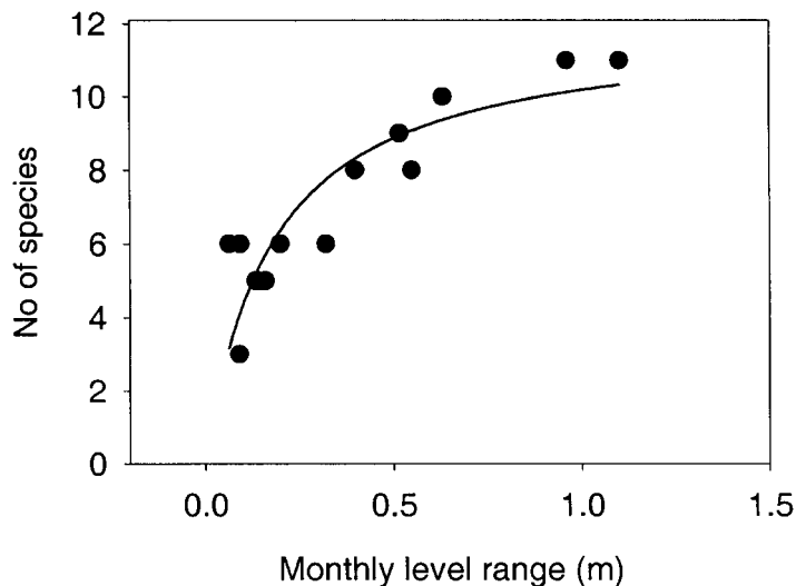
Figure 2. Relationship between water level range (mean monthly range) and the number of species of shallow water plants per lake.
