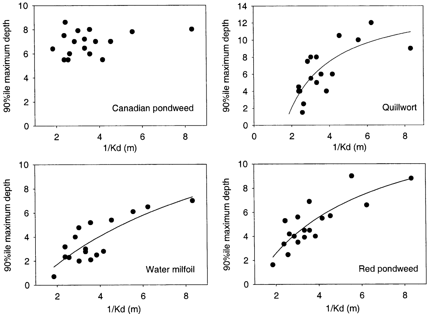
Figure 4. Significant relationships between bottom limit for most common vascular species and water clarity; the latter is expressed as the reciprocal of the attenuation coefficient of downwelling irradiance.
