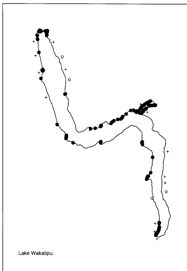
Figure 7. Predictions and observations of the locations where LMC will occur in Lake Manapouri (above) and Lake Wakatipu (below). Black dots indicate predicted occurrence, small crosses sites where LMC was found, and small circles sites where it was not.
