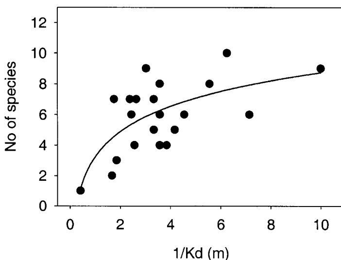
Figure 3. The relationship between water clarity and the number of species of stoneworts.
