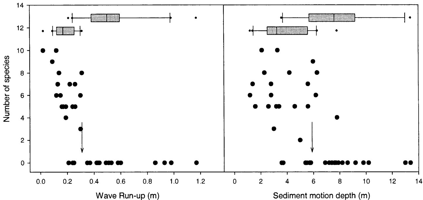
Figure 5. The relationship between wave exposure variables of wave run-up and sediment motion depth, and LMC species number. The horizontal box-whisker plots show the range, inter-quartile and median values of each exposure variable at sites with and without the LMC. Arrows designate “threshold values” for the point at which LMC becomes probable and improbable.
