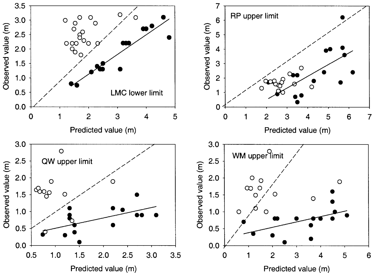
Figure 8. Observed and predicted values for the lower limits of the LMC, and the upper limits of red pondweed (RP), quillwort (QW) and NZ water milfoil (WM). Data shown for Lakes Manapouri (○) and Wakatipu (●). Broken lines show the 1:1 line, solid lines statistically significant regressions ( p < 0.05 ) for the Wakatipu data.
