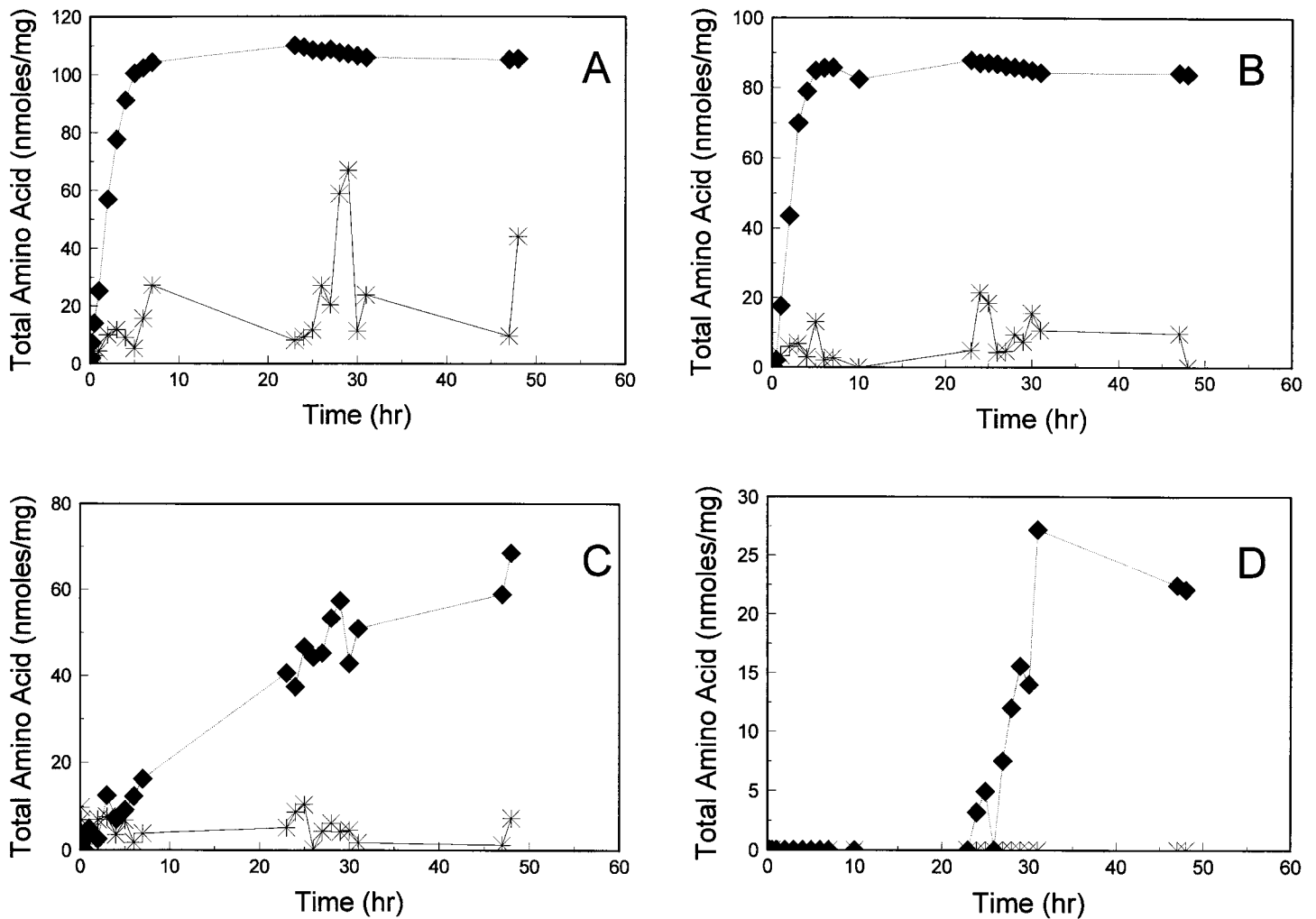
Figure 3. Time course of total amino acids leaked by hydrilla tubers (A and B) and sago pondweed tubers (C and D) exposed to 174 mmol l -1 acetic acid for 48 hours in two experiments (solid diamonds) or controls (deionized water, asterisks).
