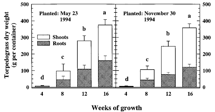
Figure 2. Dry weight of torpedograss cultured under flooded conditions with Sierra fertilizer. Each bar is the mean of four containers. Error bars are 1 standard deviation of the mean. Similar letters at the top of the bars for each date indicate no statistically significant difference for total weight at P < 0.001 according to the Waller-Duncan Bayesian procedure.
