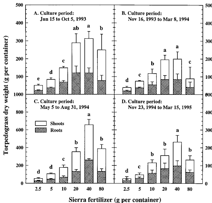
Figure 1. Dry weight of torpedograss cultured under flooded conditions with Sierra fertilizer. Each bar is the mean of four containers. Error bars are 1 standard deviation of the mean. Similar letters at the top of the bars for each date indicate no statistically significant difference for total weight at P < 0.001 according to the Waller-Duncan Bayesian procedure.
