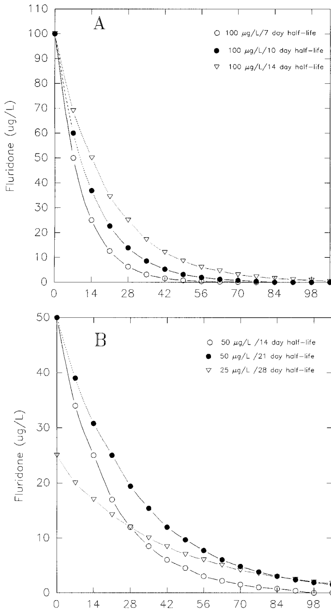
Figure 1A and 1B. Predicted dissipation of fluridone under various half-life scenarios.
