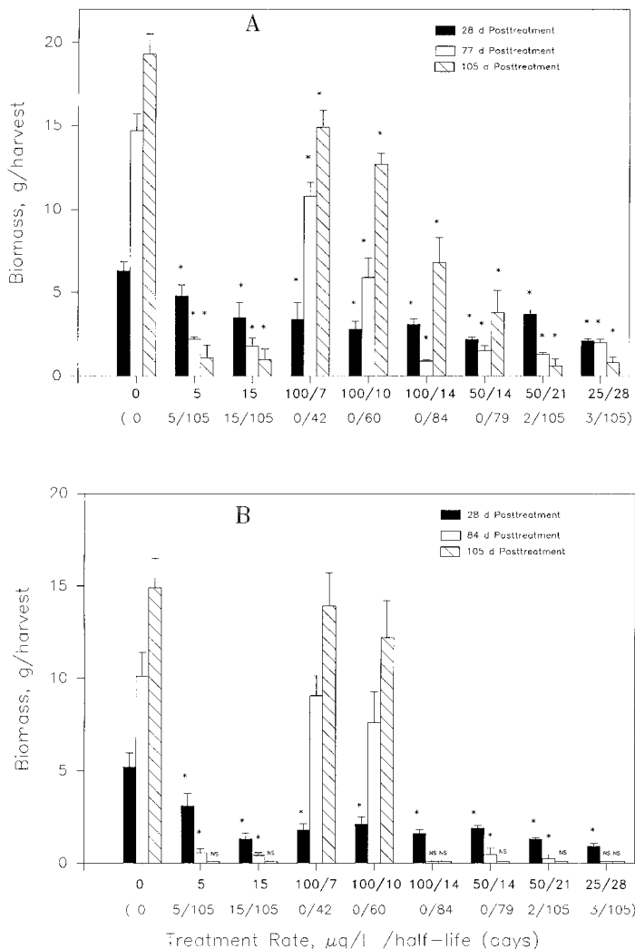
Figure 2. Effects of fluridone treatment on hydrilla (A) and Eurasian water-milfoil (B) biomass over time. Each bar represents the average of three replicates and bars with an * above them indicate treatments that are significantly different from untreated references within each sampling date according to Dunnet's test ( \alpha=0.05 ). NS indicates no sample was taken due to lack of biomass.
