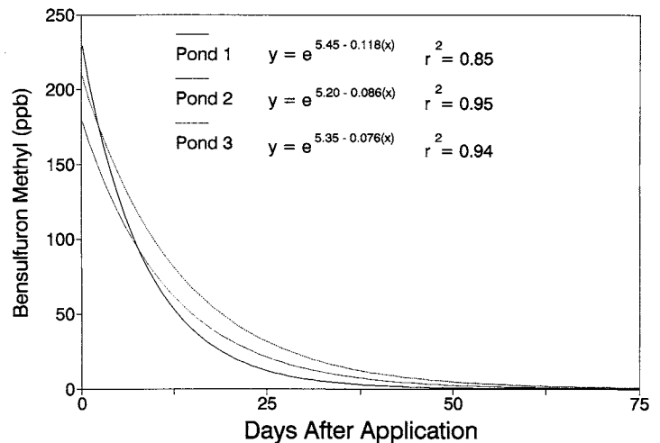
Figure 1. Concentration of bensulfuron methyl in three ponds near Welaka, Florida at various times after application.
