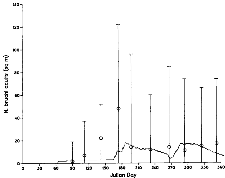
Figure 3. Simulated adult N. bruchi population plotted against the 95% confidence intervals for the 1986 North Florida site "PP" data.
