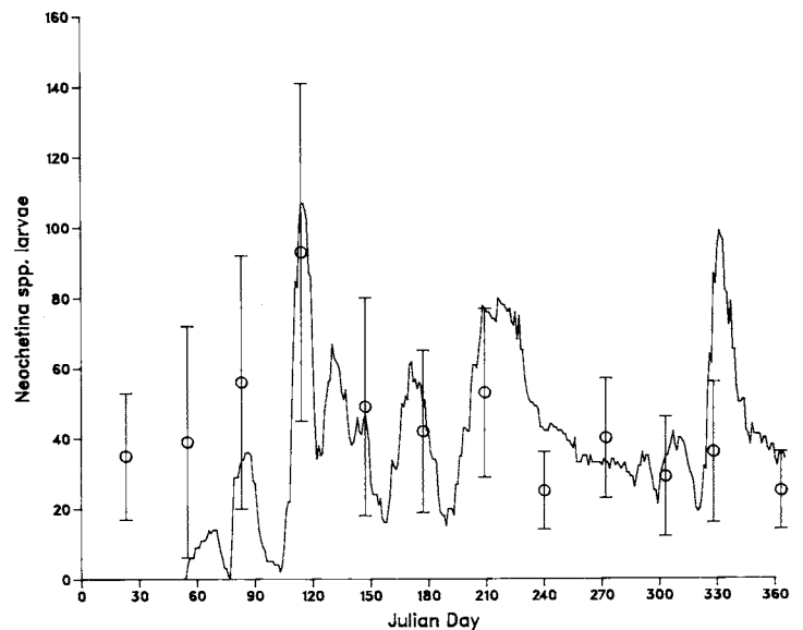
Figure 4. Simulated third instar Neochetina spp. larvae population plotted against the 95% confidence intervals for the 1986 North Florida site "CA" data.
