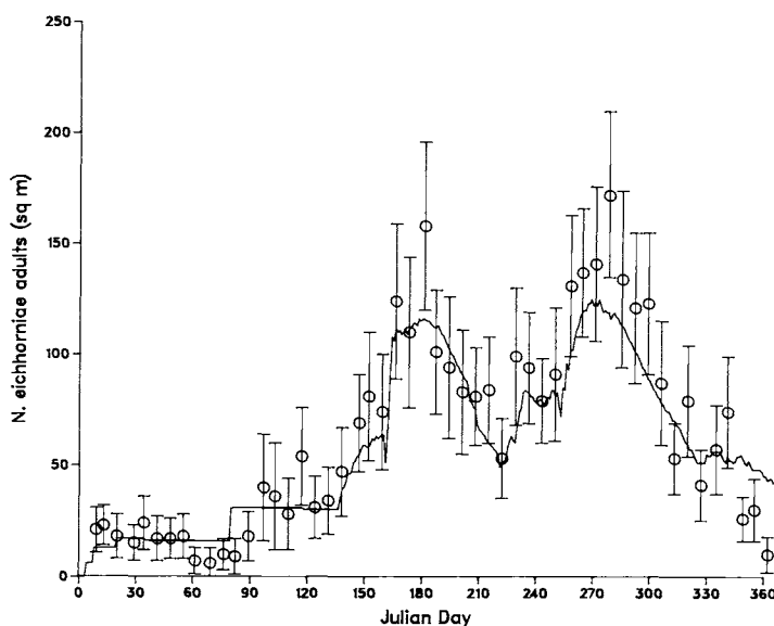
Figure 1. Simulated adult N. eichhorniae population plotted against the 95% confidence intervals for the 1976 Lake Alice data.
