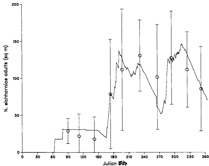
Figure 2. Simulated adult N. eichhorniae population plotted against the 95% confidence intervals for the 1986 North Florida site "PP" data.
