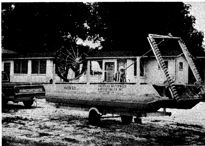
Figure 1. Mechanical weed cutter used in trials in Louisiana.
