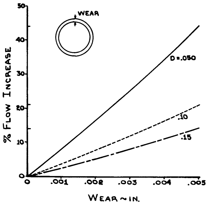
Figure 3.—Flow increase versus wear for three different size nozzles.
